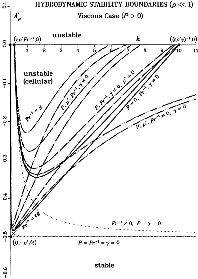
Fig. 1 Asymptotic representation of the cellular hydrodynamic neutral stability boundaries.
