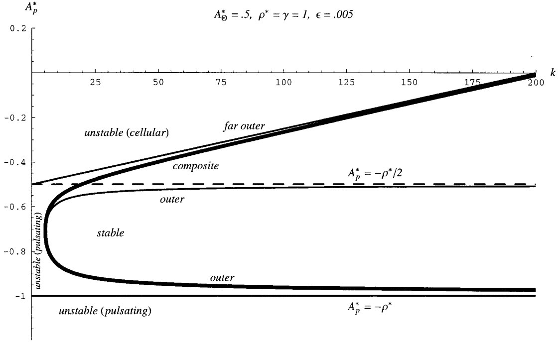
Fig. 3 Composite pulsating/cellular hydrodynamic stability boundary for A_\Theta \sim \mathcal{O}(\epsilon^{1/4}) in the limit of zero viscosity.
