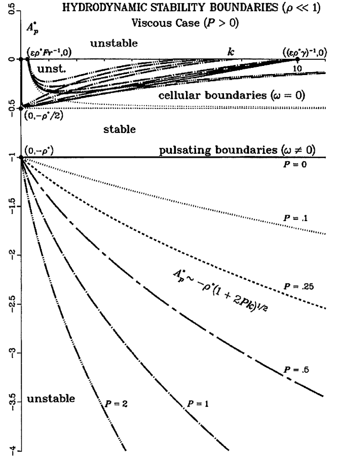
Fig. 2 Asymptotic representation of the pulsating hydrodynamic stability boundary for the viscous case ( P > 0 ). The cellular boundaries are the same as shown in Fig. 1.
