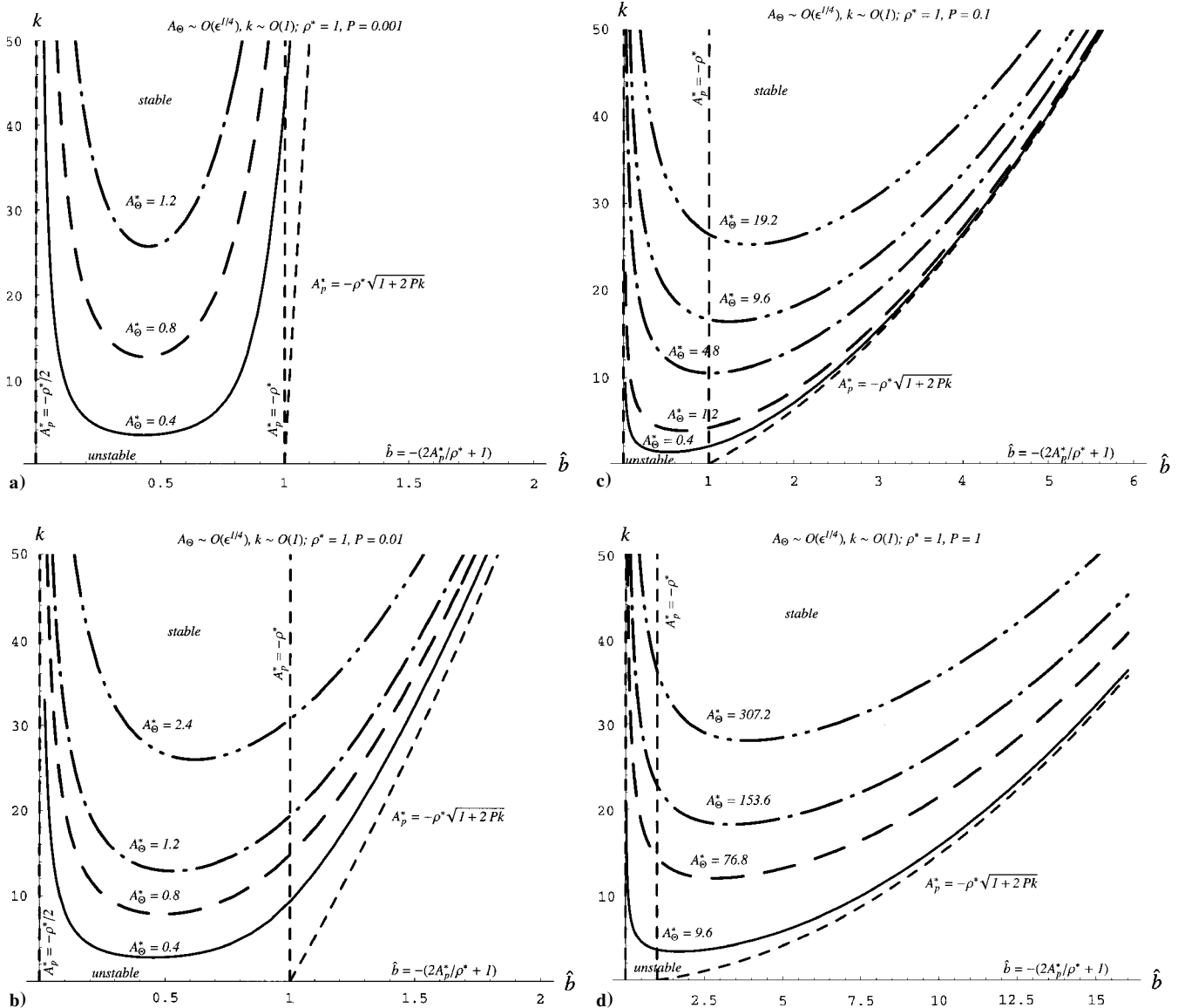
Fig. 4 Pulsating hydrodynamic stability boundaries for k \sim \mathcal{O}(1) and A_\Theta \sim \mathcal{O}(\epsilon^{1/4}) in the general viscous case for \rho^* = 1 and a) P = .001 , b) P = 0.01 , c) P = 0.1 , and d) P = 1.0 .
