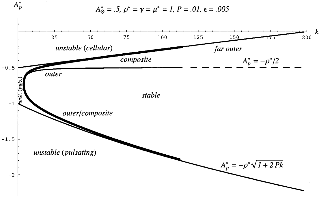
Fig. 5 Composite pulsating/cellular hydrodynamic stability boundary for A_\Theta \sim \mathcal{O}(\epsilon^{1/4}) in the general viscous case.
